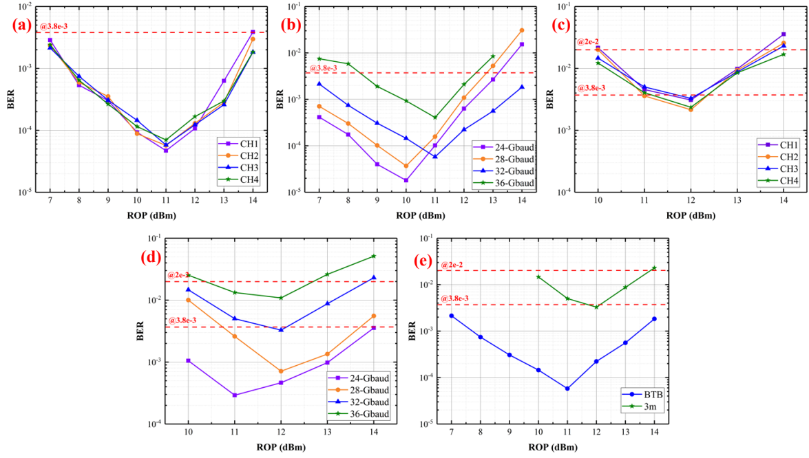
Fig. 2: (a) BER versus ROP of four channels with a rate of 32Gbaud in the BtB scenario; (b) BER versus ROP of CH3 with rates of 24-, 28-, 32-, and 36-Gbaud in the BtB scenario; (c) BER versus ROP of four channels with a rate of 32Gbaud in the 3 m scenario; (d) BER versus ROP of CH3 with rates of 24-, 28-, 32-, and 36-Gbaud in the 3 m scenario; (e) BER versus ROP of CH3 with a rates of 32Gbaud in the BtB and 3 m scenarios
