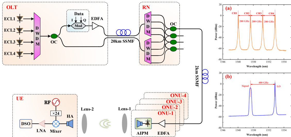
Fig. 1: Experimental setup of simplified point-to-multipoint photonics-assisted ToF-PON architecture. Optical spectra: (a) the four CWs; (b) the optical carrier and LO after optical coupler
