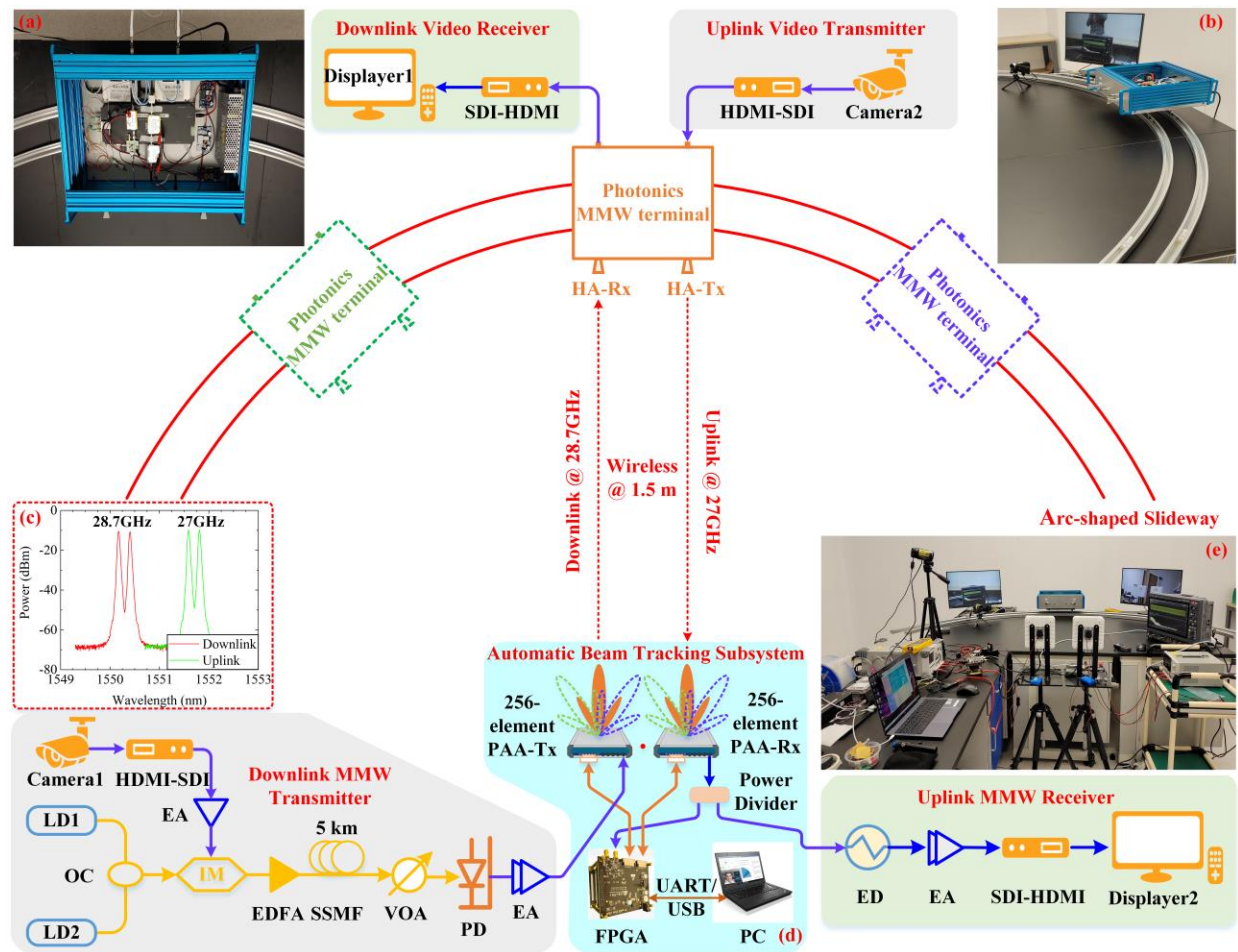
Fig. 1. Demonstration setup of real-time bi-directional HD video transmissions based on 5G MMW PAAs. (a) Packaged chassis of the photonics MMW terminal. (b) Arc-shaped slideway. (c) Optical spectra of the uplink and downlink. (d) Automatic beam tracking subsystem; (e) Testbed.
