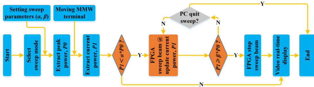
Fig. 2. Automatic beam tracking workflow.
